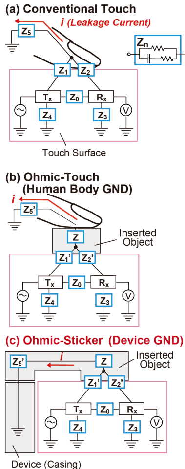
Figure 3: Equivalent circuit of capacitive touch surfaces. (a) Conventional touch; (b) Ohmic-Touch [5]: human body GND; (c) Ohmic-Sticker: connecting the object to the device casing.
