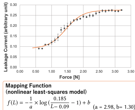
Figure 8: Mean leakage current for press input; Orange line: The mapping function.
