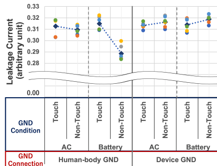
Figure 5: Mean leakage current for each GND condition and GND connection method. (P: participant)
