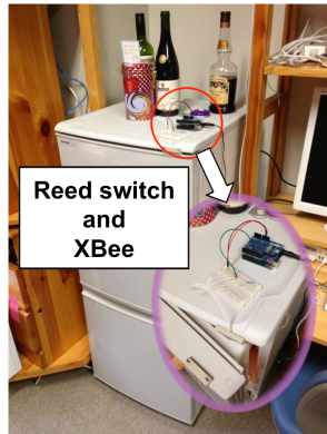
Figure 4: Refrigerator hardware. Xbee and reed switch.
