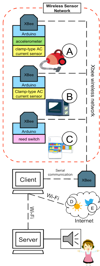
Figure 2: System composition. (A) vacuum cleaner, (B) microwave, (C) refrigerator, (D) weather report, (E) Twitter.
