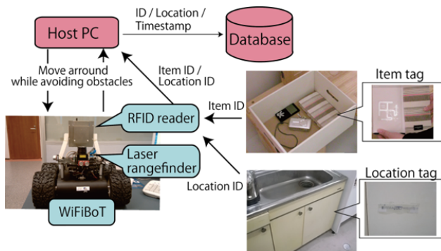
Figure 2. The system architecture of IteMinder
