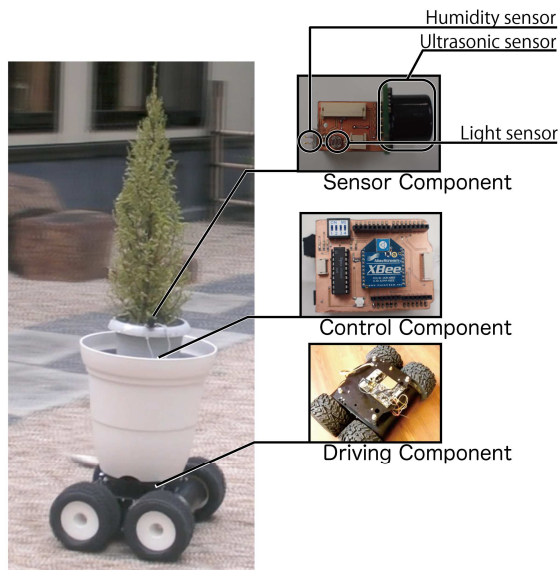
Figure 3. The PotPet prototype.
