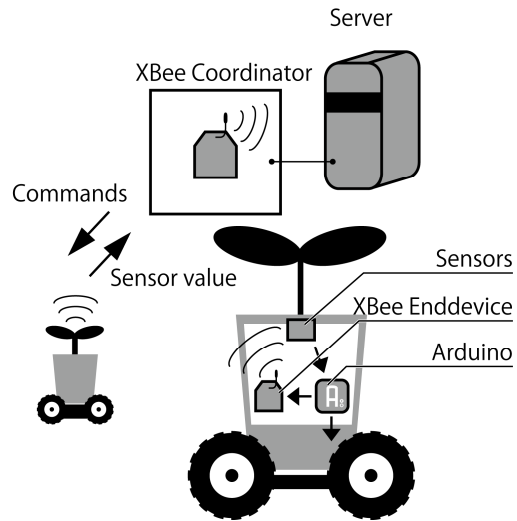
Figure 4. The system architecture of the PotPet.
